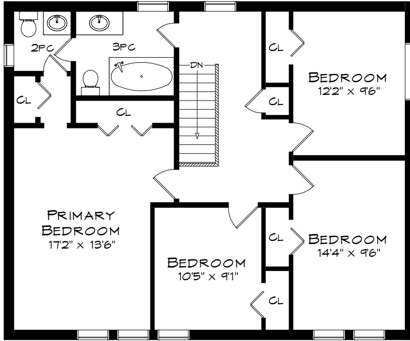
UPPER LEVEL 1,002 SQUARE FEET
